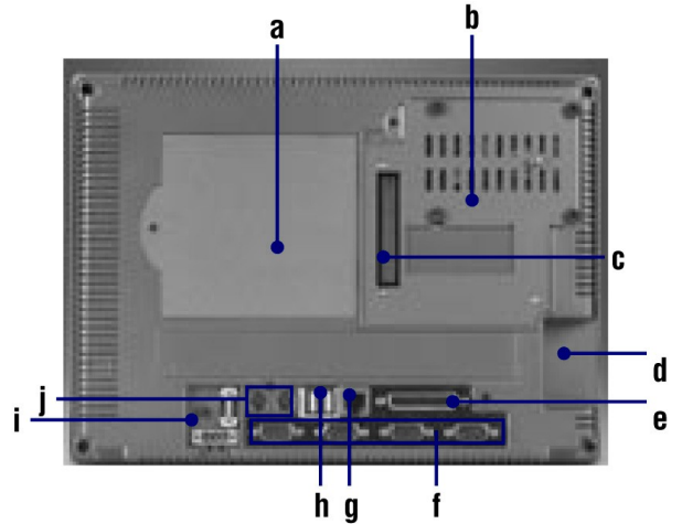
SSH-12X, 12XL Rear View
