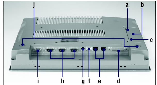
SSH-15x Rear View
