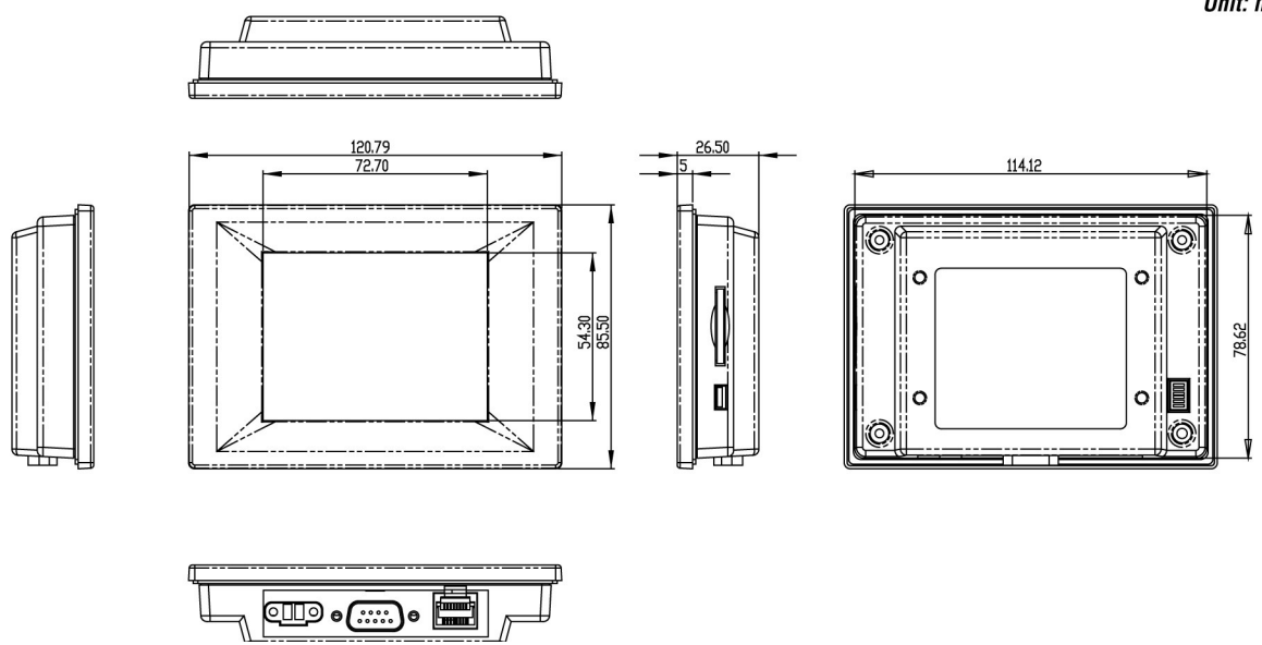
SSH-30Cx Mounting Diagram
