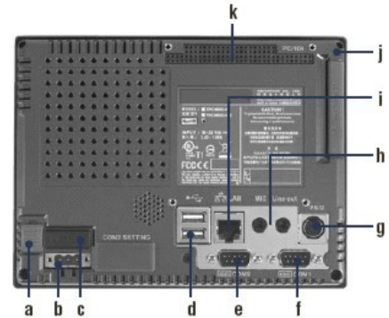
SSH-60x Rear View
