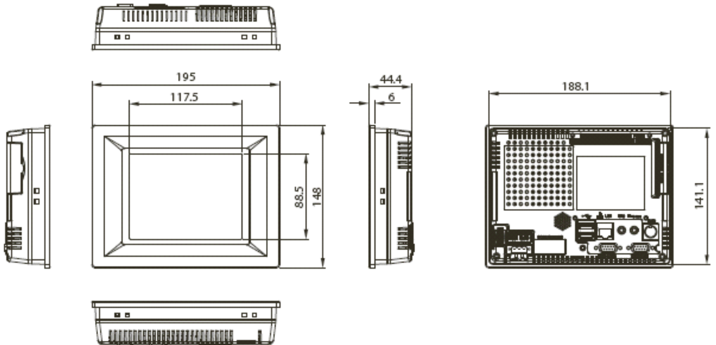
SSH-60x Mounting Diagram
